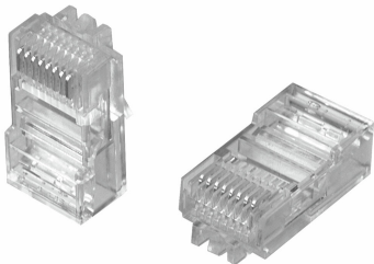
Modular Plug Kit, 8P/8C, unshielded, flat oval, 2.54 x 8.89 mm max cable jack OD, 8-position, 100/bag
